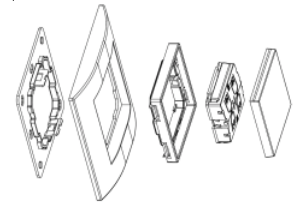
Central plate, design frame (not included), intermediate frame, wall transmitter, actuating rocker(s)
